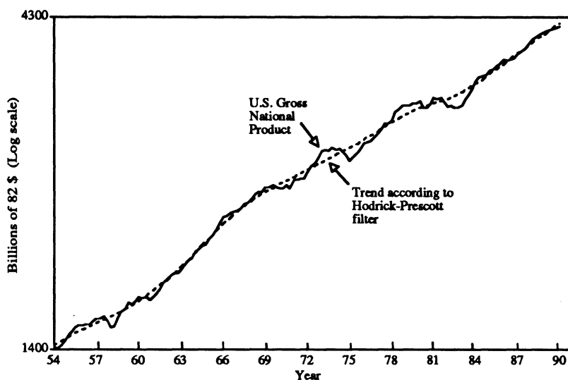
FIG. 1.—Example of a U.S. time series detrended with the Hodrick-Prscott filter. Source: Citibase.
